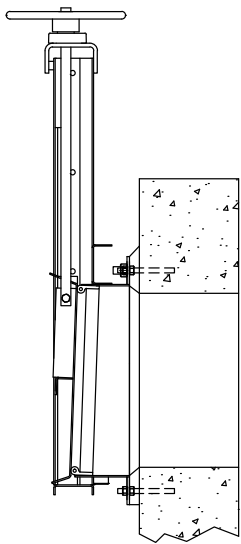
WALL MOUNTED
